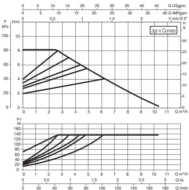
EVOPLUS 80/180 XM
